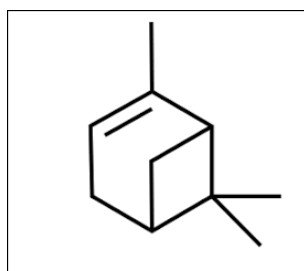
Fig.2: Structure of Pinene
