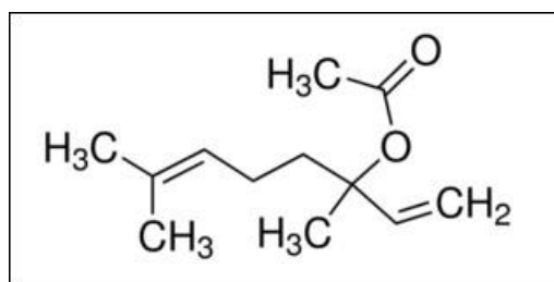
Fig.12: Structure of Linayl acetate
