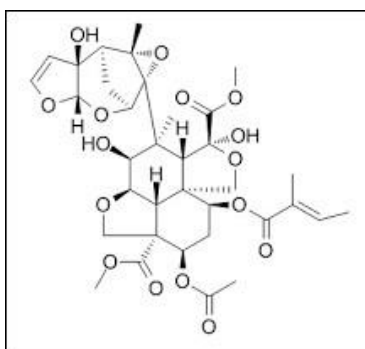
Fig.8: Structure of Azadirachtin
