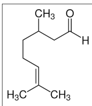
Fig. 4: Structure of citronellal
